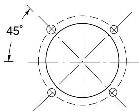
Flange Max-3 (250-320) 4 x M10 (45°)
